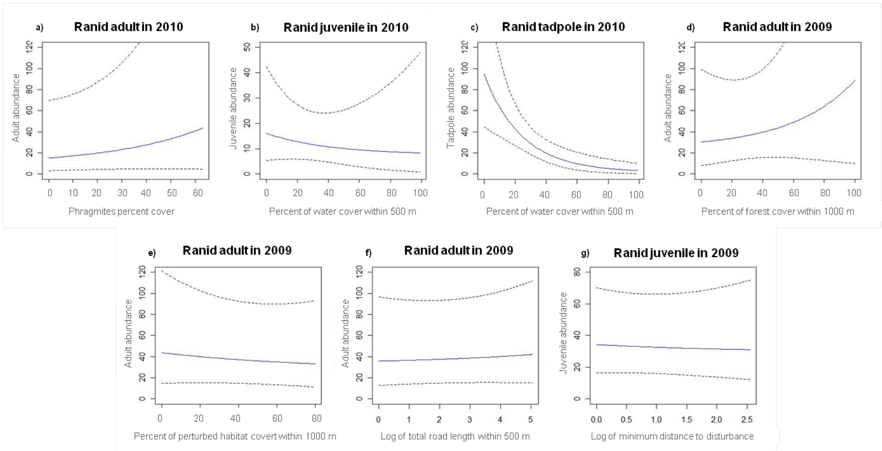
Fig 2: Model-averaged ranid abundance as a function of wetland and landscape scale variables from trapping data in 50 wetlands of the Montréal area, Québec, Canada in 2009 and 2010. Dashed lines indicate 95% unconditional confidence interval around predictions.
